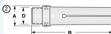
Style "AF" Master Feed Finger Pad
