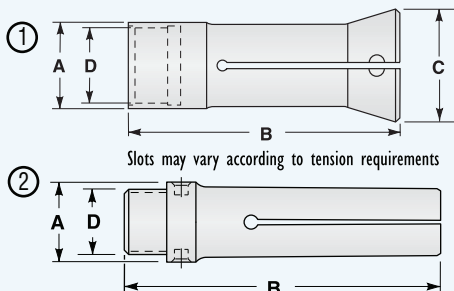
Style "S" Master Collet & Pad
