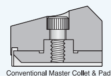
Conventional Master Collet & Pad
