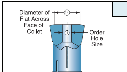
Chamfer - Diameter
