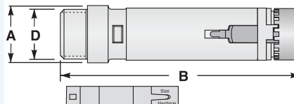
Style "AF" Master Feed Finger Pad
